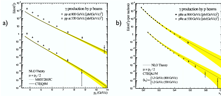
Fig. 2. E706 results compared with pQCD. a) pp \rightarrow \gamma X vs. p_t , b) pBe \rightarrow \gamma X vs. x_t = 2p_t/\sqrt{s} with k_t smearing.
